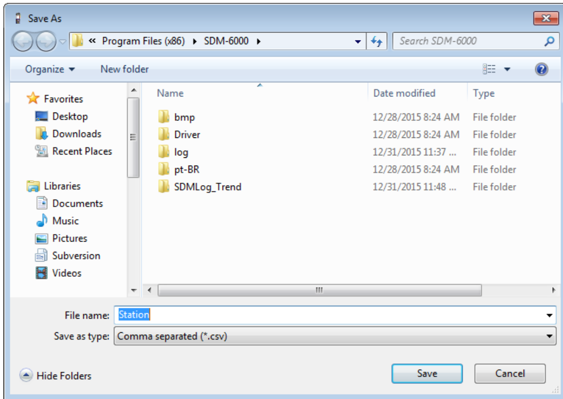
Figure 113: Save As
