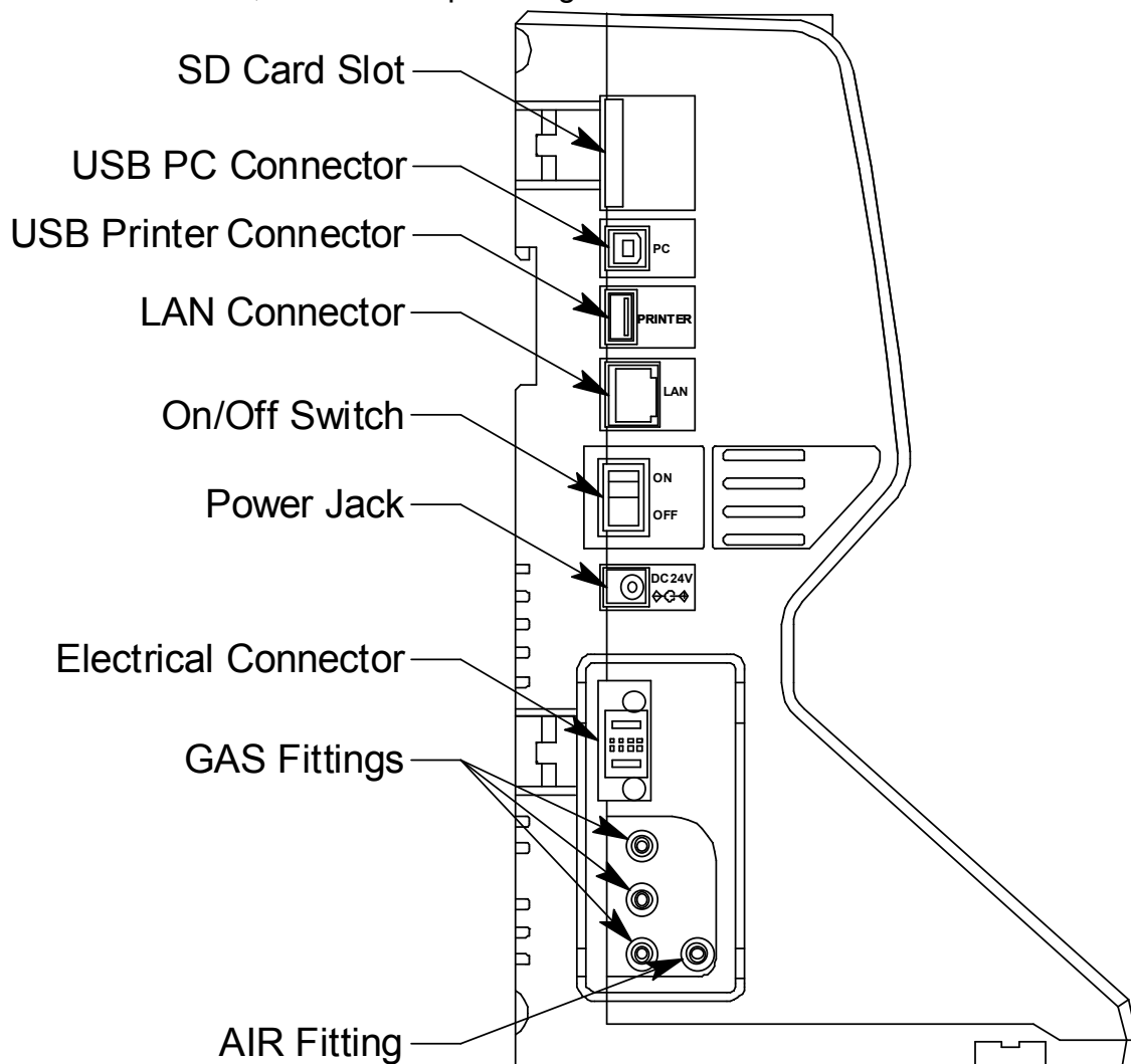
Figure 4: Left Panel Component Location
