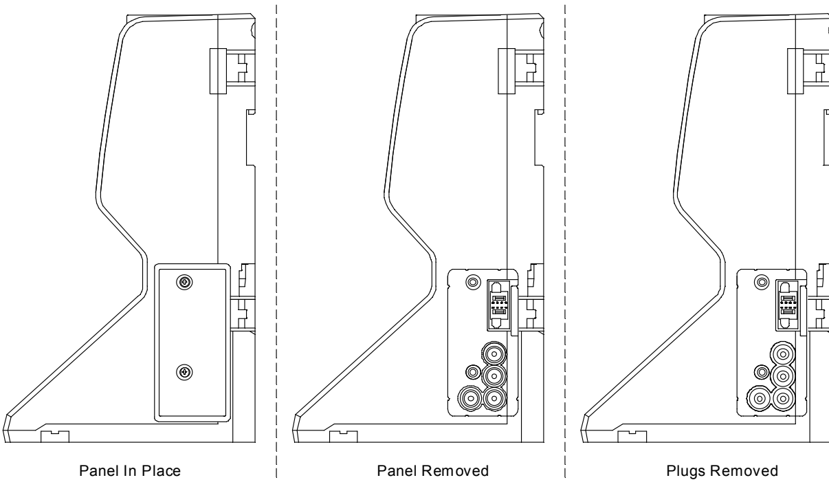
Figure 12: Panel and Plug Removal
