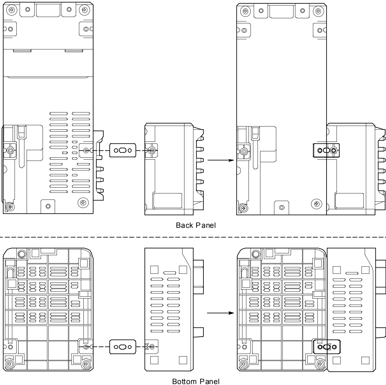
Figure 15: Connecting the SV-3
