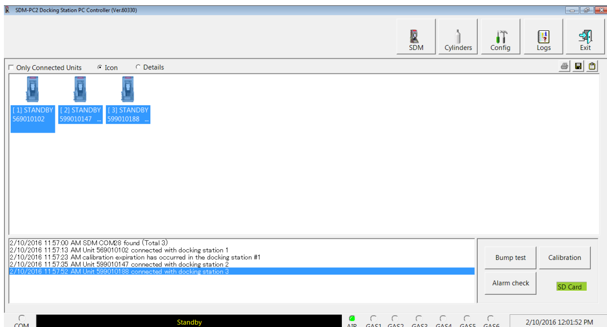
Figure 47: Instrument Selection
