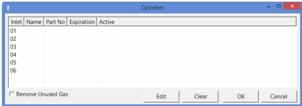
Figure 27: Cylinders Window
