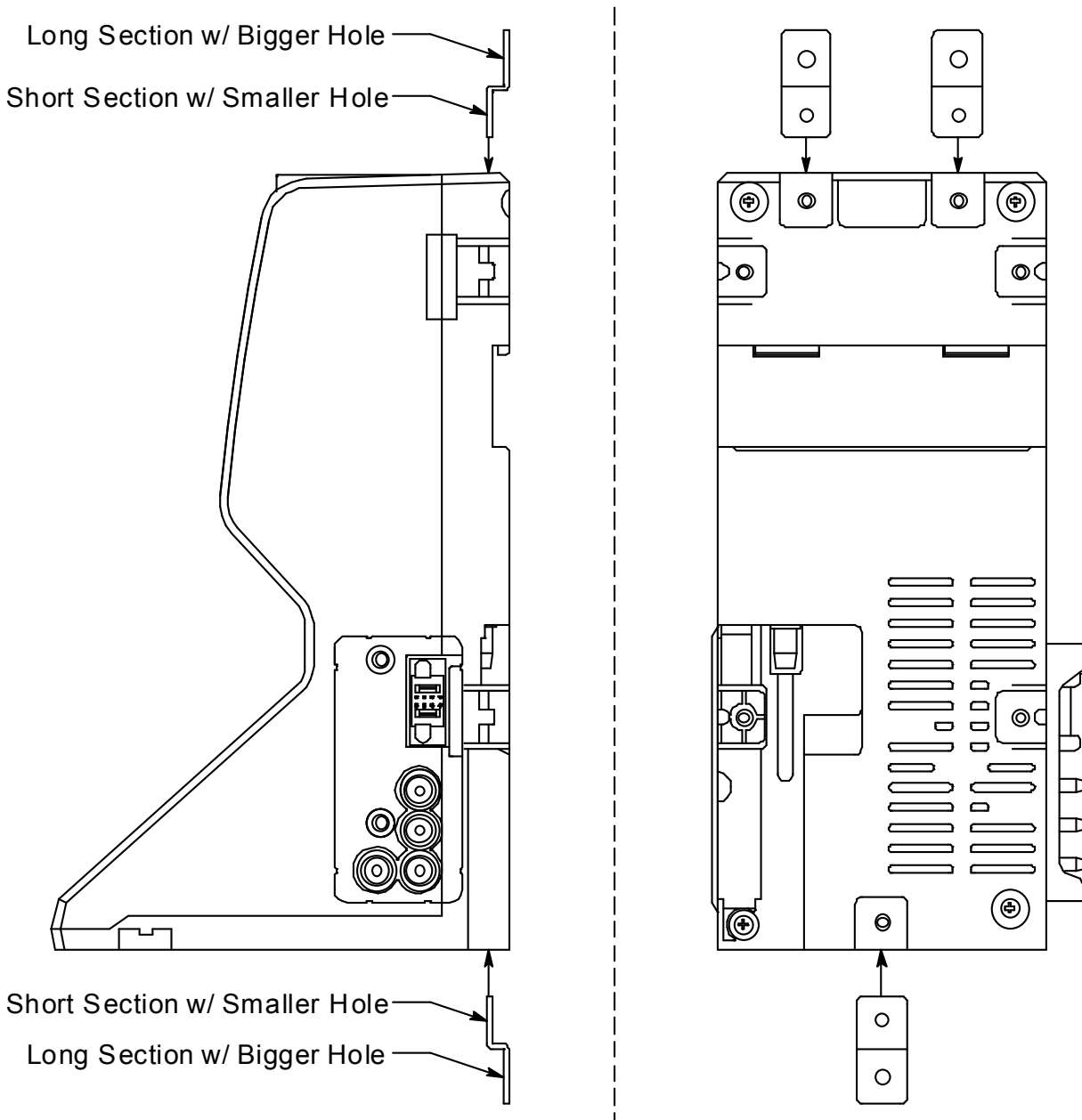
Figure 18: Wall Mounting Bracket Installation
