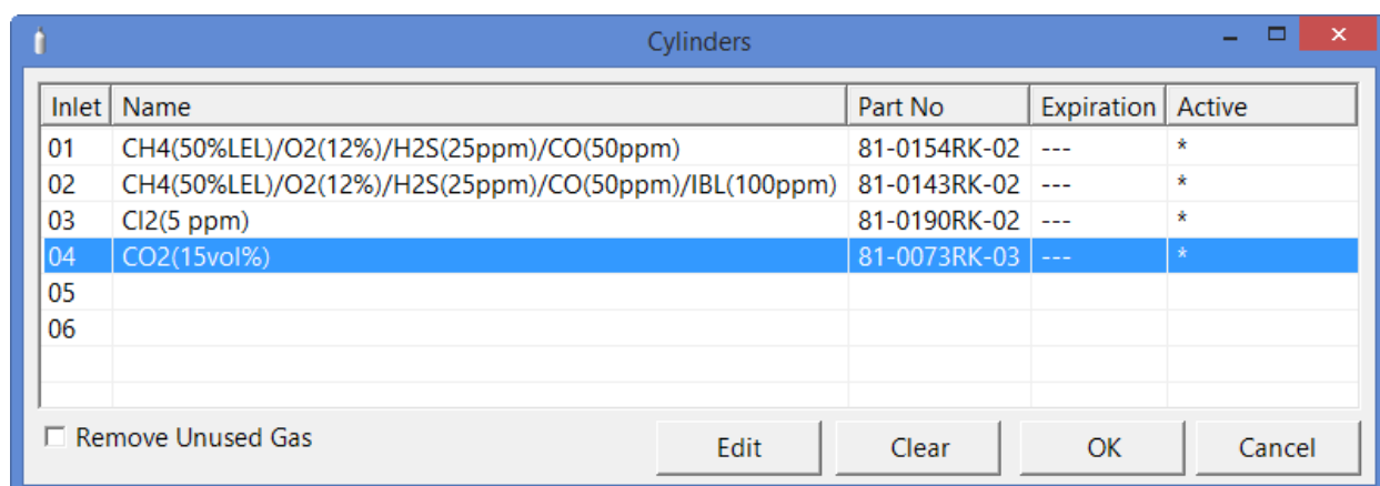
Figure 38: Cylinder Selected
