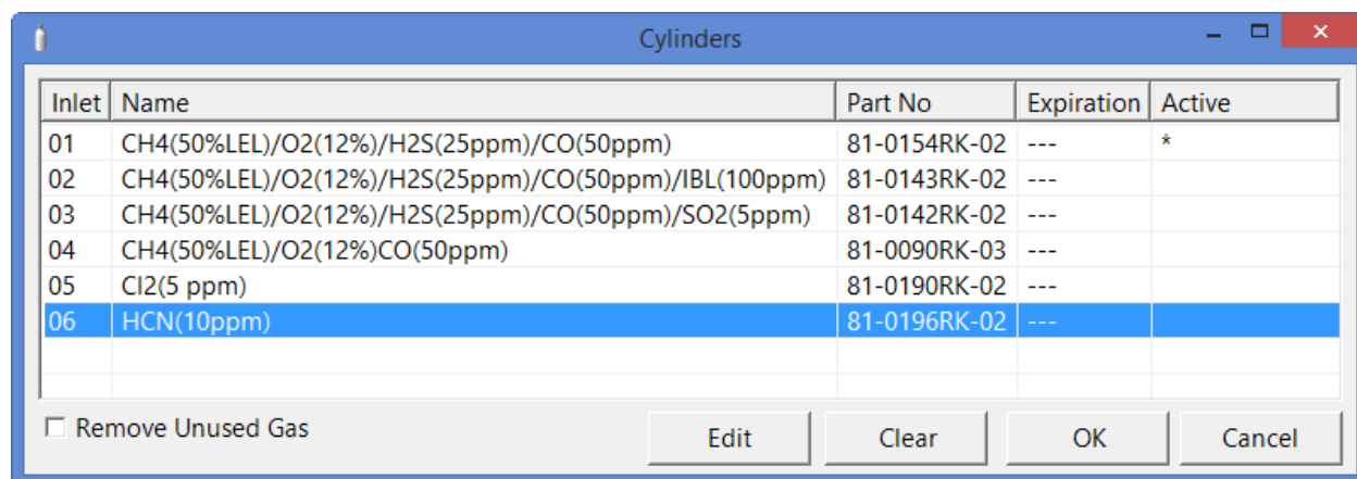
Figure 37: Cylinders Window
