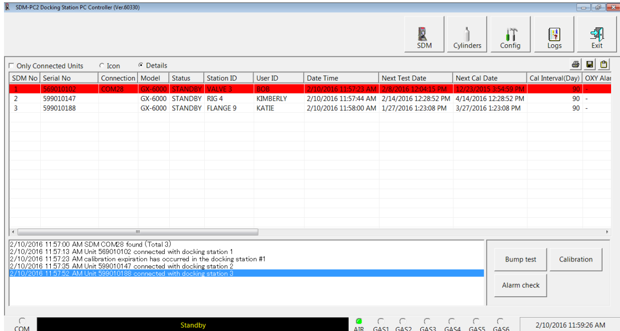
Figure 46: Details View
