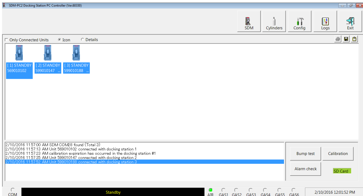
Figure 64: Instrument Selection
