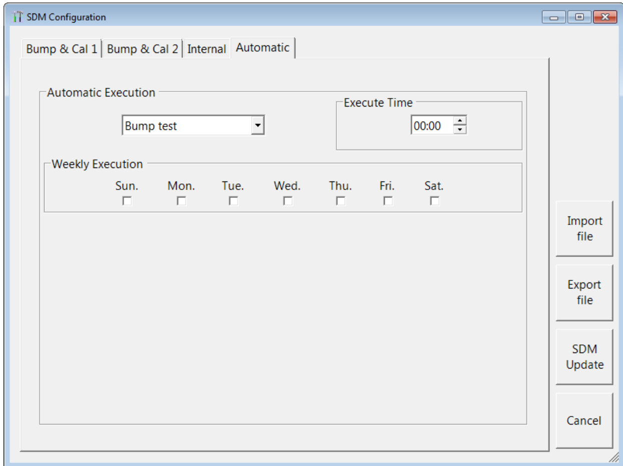
Figure 26: Automatic Tab
