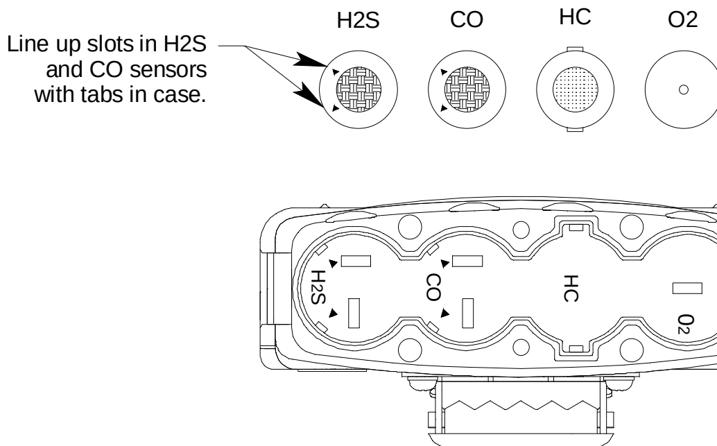
Figure 23: Replacing the Sensors and Their Locations in the GX-2009
