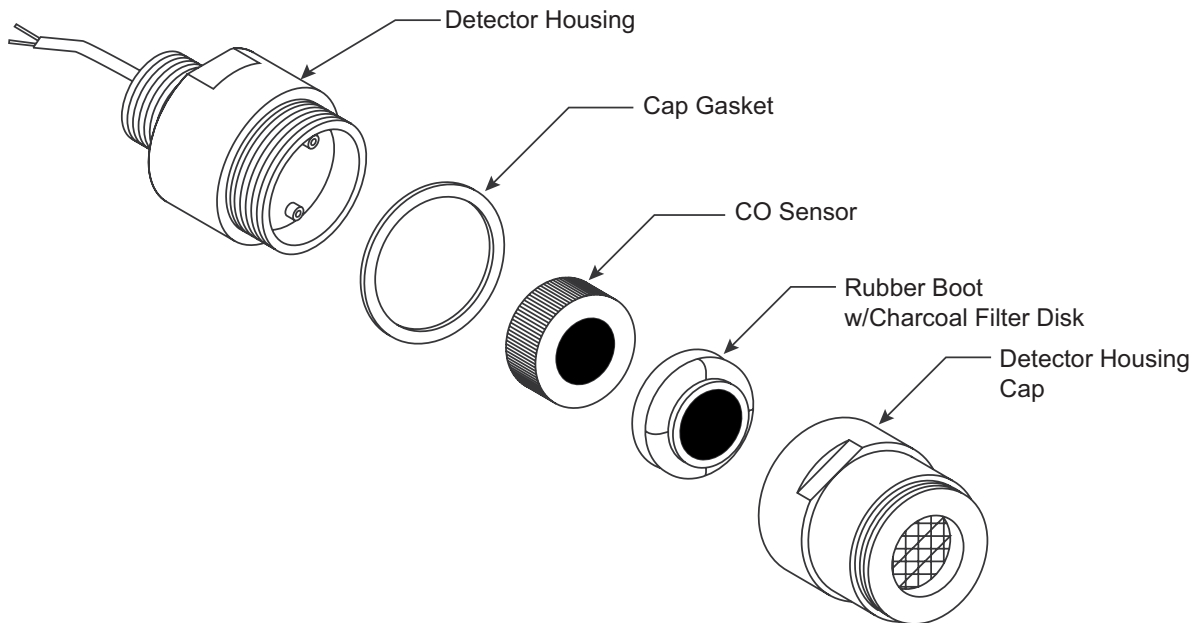
Figure 3: 65-2433RK-05CO Detector
