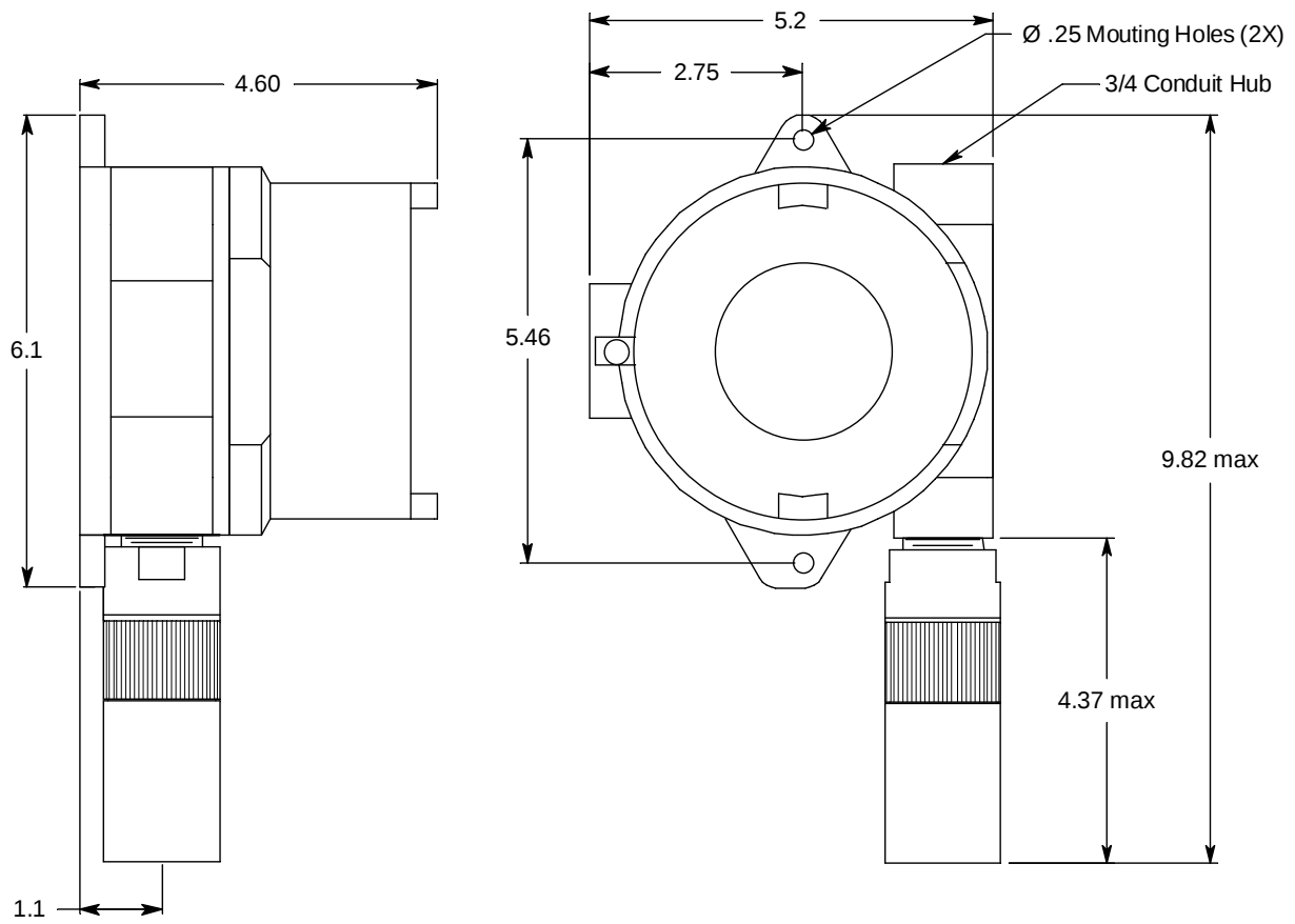
Figure 13: Outline & Mounting Dimensions, ESM-01 Toxic
