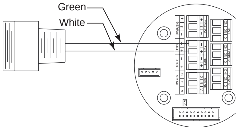
Figure 17: Capillary Oxygen Detector Wiring
