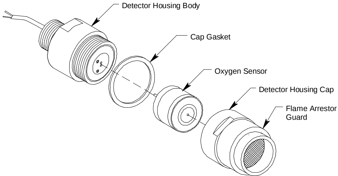
Figure 2: 65-2514RK Oxygen detector
