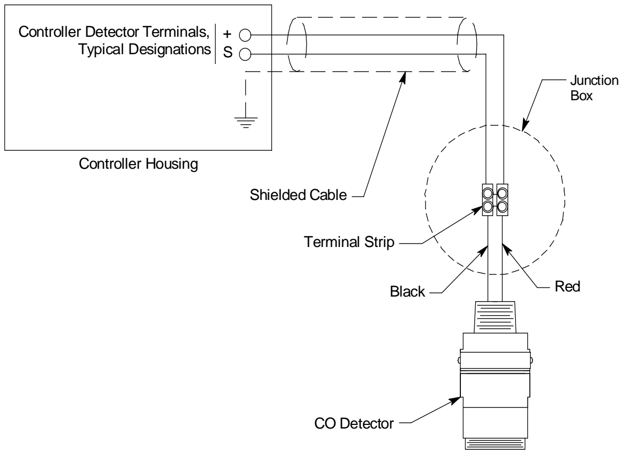
Figure 3: Wiring the CO Detector to a Controller
