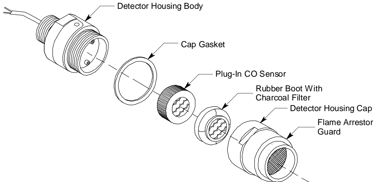
Figure 1: CO Detector Component Location
