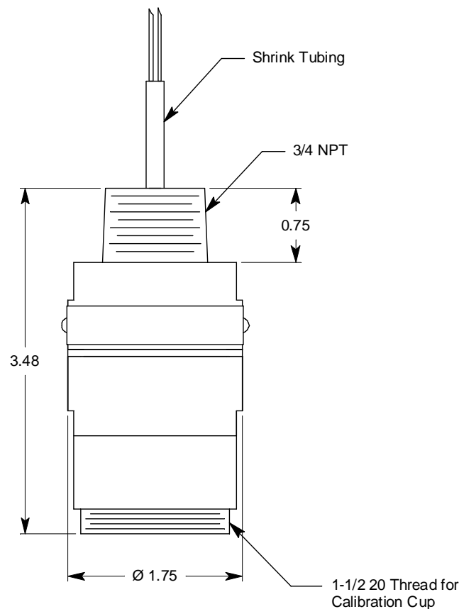
Figure 2: Outline & Mounting Dimensions
