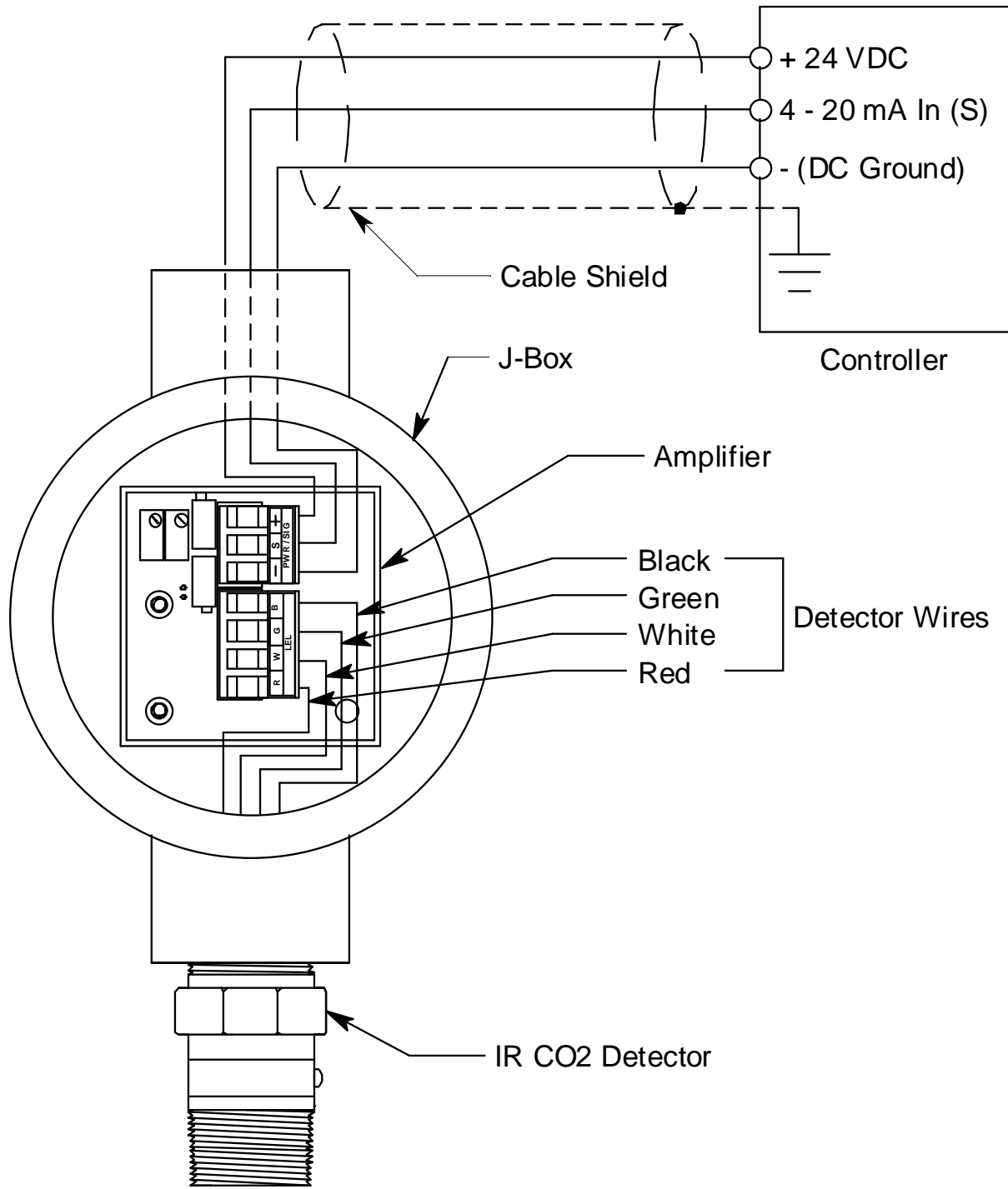
Figure 3: Wiring the CO 2 Transmitter to a Controller
