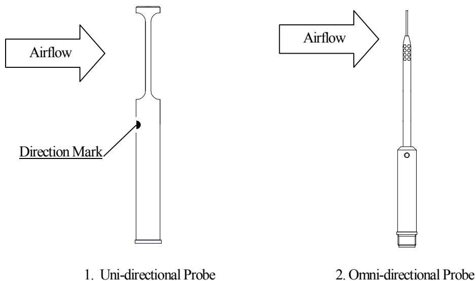
Probe Direction
