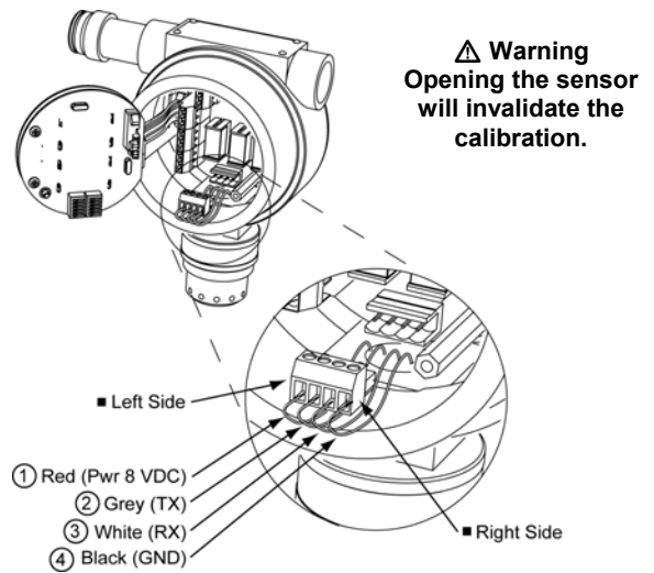
Figure 9. Sensor Wiring Diagram
